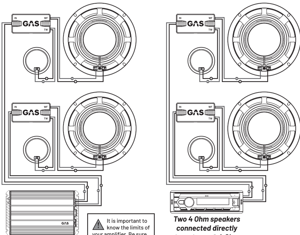
Two 4 Ohm speakers connected with an amplifier @ 4 Ohm
